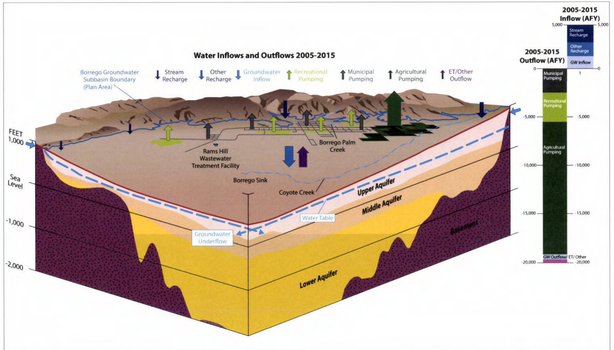
FIGURE 2.2-1 Hydrogeological Conceptual Model of the Plan Area Groundwater Sustainability Plan for the Borrego Springs Groundwater Subbasin
